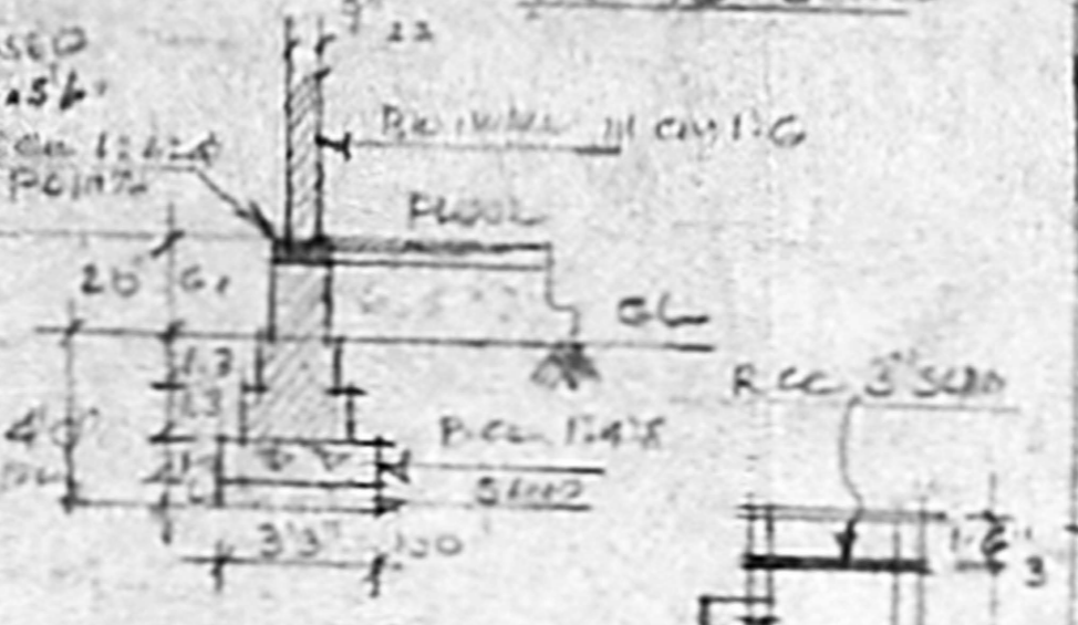
DETAILS OF WALL FOUNDATION AT (C)
